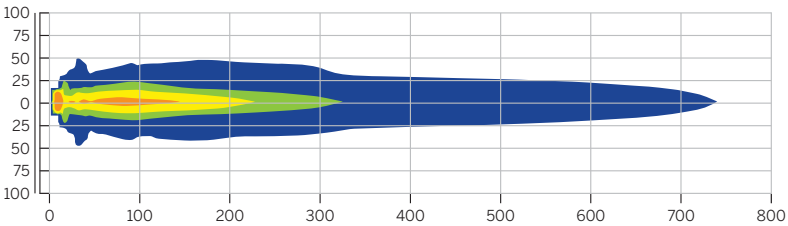
Dual Bulb Halogen Headlamp High Beam (7") Birds Eye View (shown in feet)
