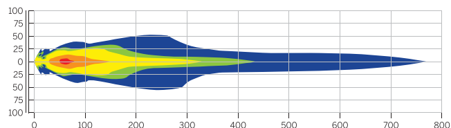
Daymaker Reflector LED Headlamp – High Beam (7") Birds Eye View (shown in feet)
