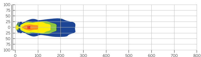
Daymaker Reflector LED Headlamp – Low Beam (7") Birds Eye View (shown in feet)
