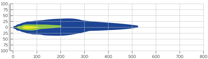
Original Equipment Headlamp High Beam (7") Birds Eye View (shown in feet)
